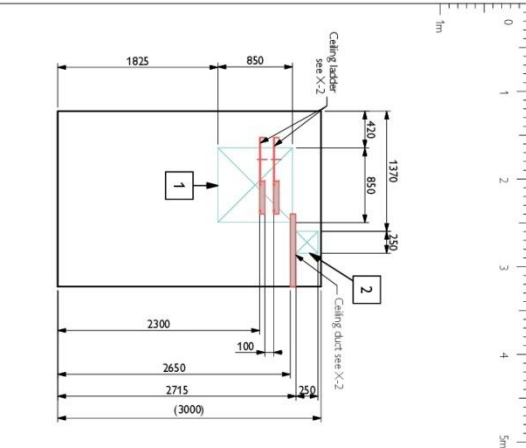
Elevation C
