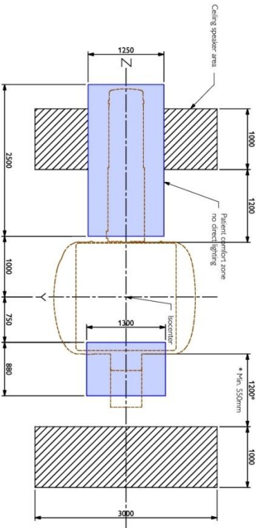
Detail - Ceiling area for lighting and speakers (scale 1:50)
