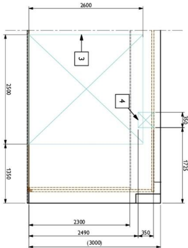
Elevation D
